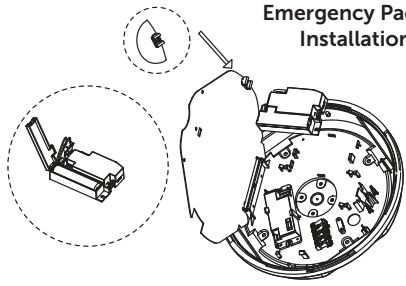
Connection PWM + Emergency Pack
