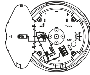
Connection PWM
