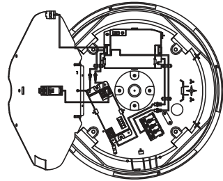
Connection PWM + Emergency Pack
